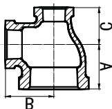
Reducing Tee
